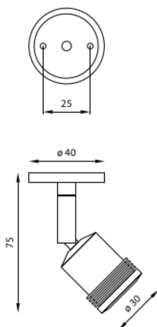
Alle Maße in mm | All dimensions in mm
