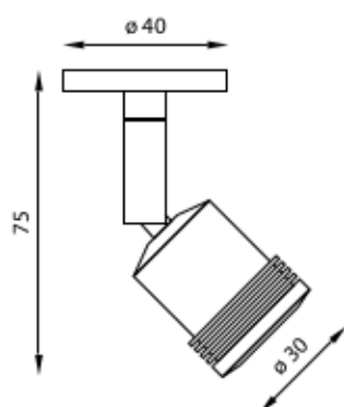
Alle Maße in mm | All dimensions in mm
